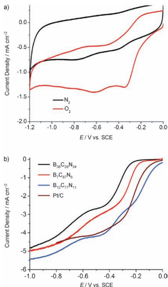
Figure 3. a) Cyclic voltammetry (CV) curves of ORR on BCN ( B_{12}C_{77}N_{11} ) graphene in nitrogen- and oxygen-saturated 0.1 M KOH solutions at a scan rate of 50 mVs -1 . b) LSV curves of ORR on BCN graphene with different compositions in oxygen-saturated 0.1 M KOH solution at 10 mVs -1 and compared with the commercial Pt/C electrocatalyst.
